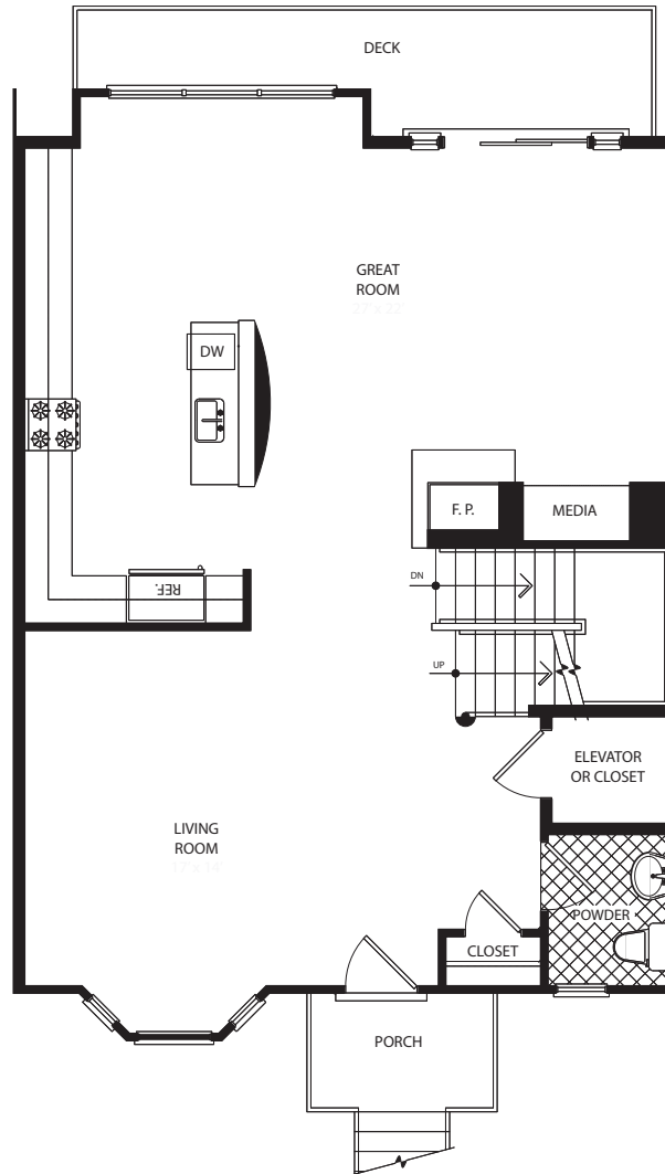
MARINER'S WALK E FIRST FLOOR
